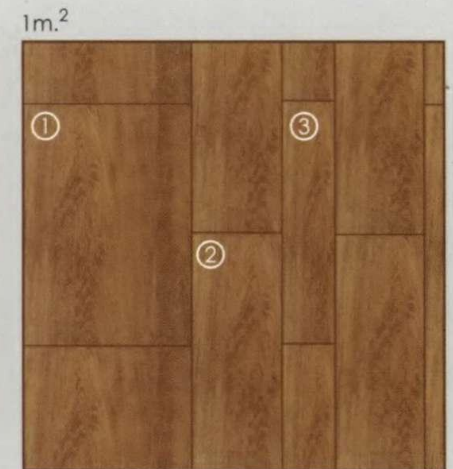
Teak 1. Teak 195 X 585 mm. 35% 2. Teak 392 X 585 mm. 40% 3. Teak 96 X 585 mm. 25%
